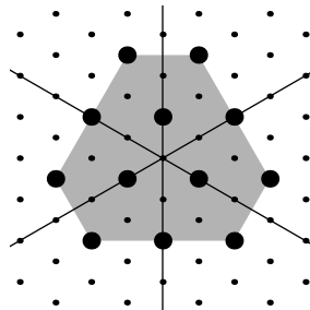
Figure 8.1. Set of weights of a representation V of Lie algebra \mathfrak{sl}(3, \mathbb{C}) . Large dots are the weights of V , small dots are all weights \lambda \in P ; shaded area is the convex hull of P(V) . The figure also shows the root hyperplanes.
